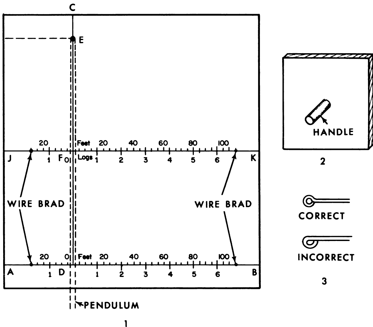
Figure 2-3. Construction of the modified Faustman hypsometer.
